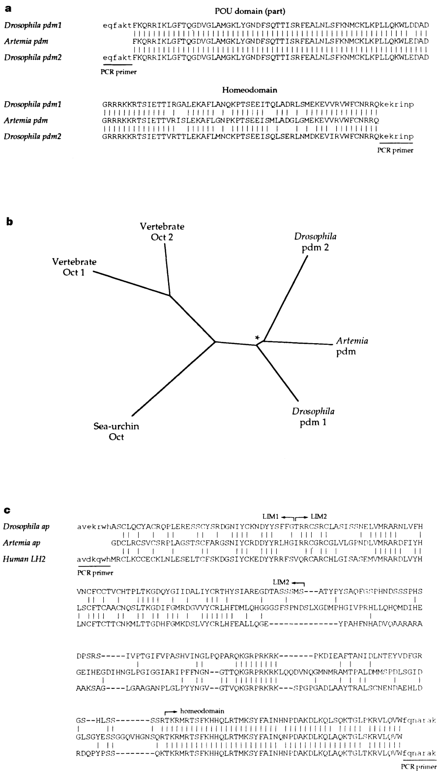
Figure 2 a , Sequence alignment of Af-PDM with its Drosophila counterparts Pdm1 and Pdm2. Alignments are shown for the POU domain and homeodomain regions only; no significant sequence similarity was found outside these regions. Amino-acid identity is indicated by a vertical line. The positions of PCR primers used for the isolation of the Artemia gene (see Methods) are shown. b , Tree depicting the sequence relationships of Af-pdm with Drosophila pdm1 and pdm2 , and their counterparts from vertebrates and sea urchins (Oct genes). Comparisons were made at the amino-acid level on the available POU and homeodomain sequences only (as in a ). The node between Af-pdm , pdm1 and pdm2 (marked by
