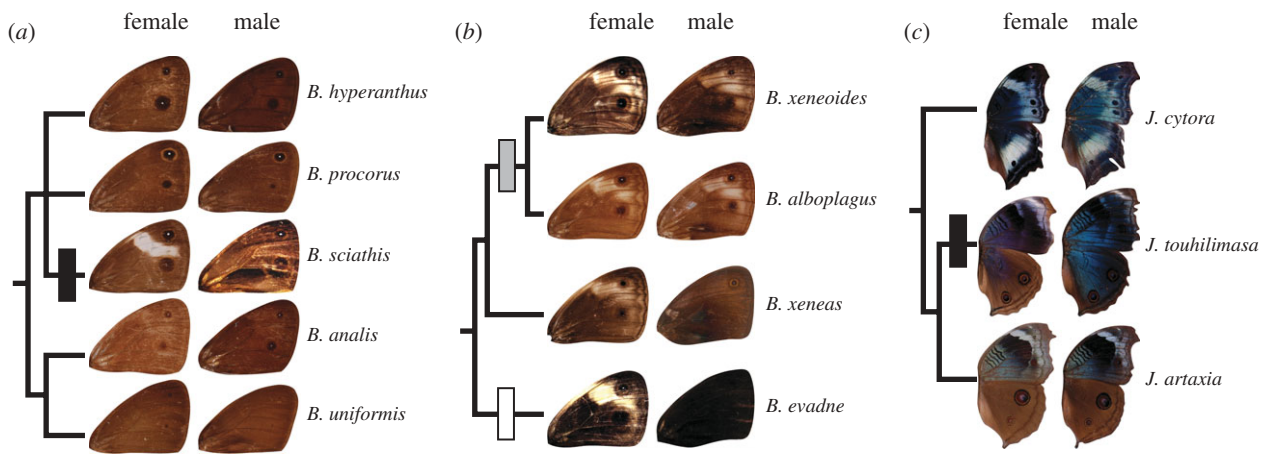
Figure 2. Examples of sexual dimorphism evolution in Bicyclus and Junonia . (a) Single sex gain (SSG): the sub-apical band was gained by females alone in the lineage leading to B. sciathis . (b) Single sex loss (SSL): male expression of the M_1 eyespot was lost in the lineage leading to B. evadne (white bar). (c) SSG: the distal shutter was gained by males alone in the lineage leading to Junonia touhilimasa . The grey bar in (b) highlights conversion of female-limited expression of the sub-apical band to dual-sex expression in the lineage ancestral to B. alboplagus and B. xeneoides .
